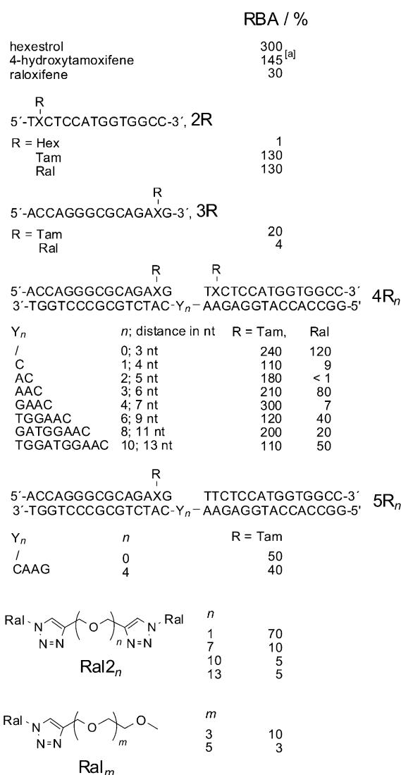
Figure 2. Relative binding affinity (RBA, relative to estradiol). [a] Calculated for a 1:1 mixture of the cis/trans isomers. nt = nucleotide. (Conditions: see Table S4 in the Supporting Information.)
